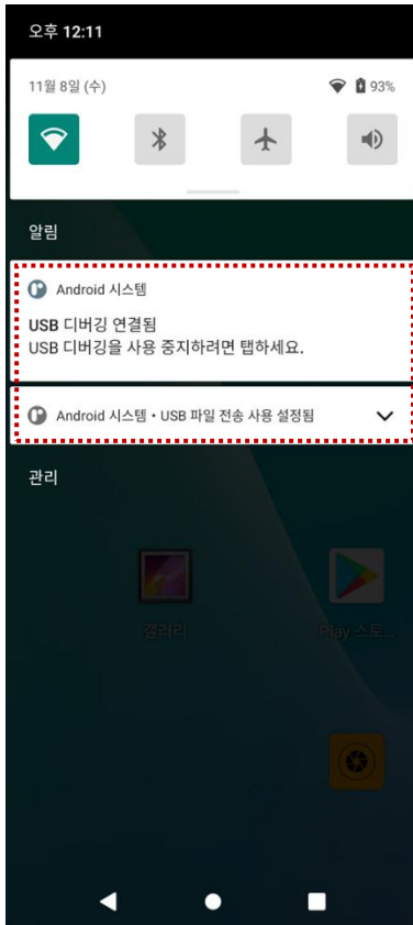
Figure 18 알림창
