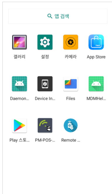
Figure 22 앱 서랍
